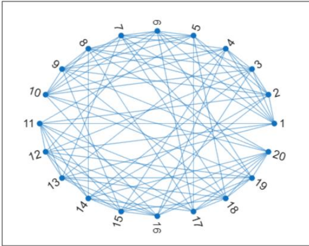
Johnson graph J(6,3)
